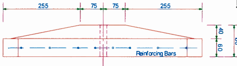
FRONT ELEVATION
