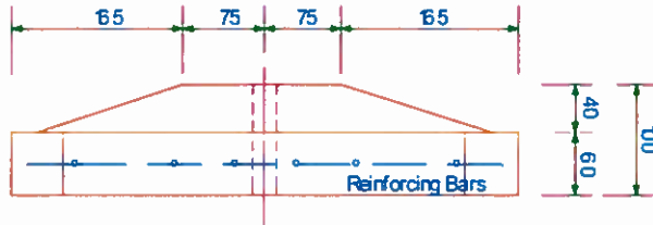
SIDE ELEVATION
