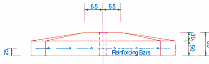
FRONT ELEVATION
